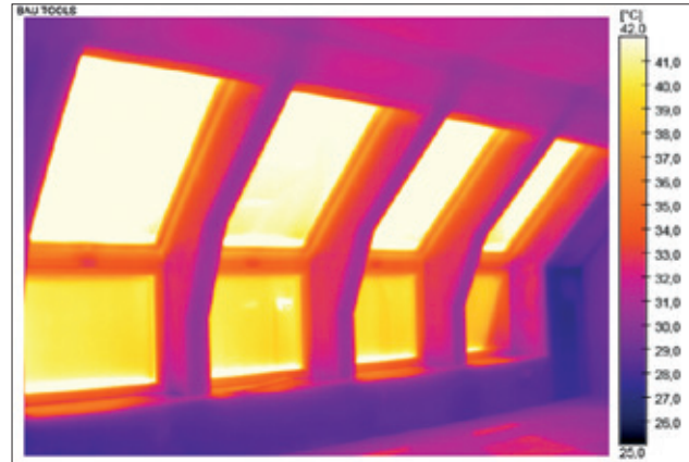
Sunlit window: Thermogram "starting image" BauTools BlowerDoor.
